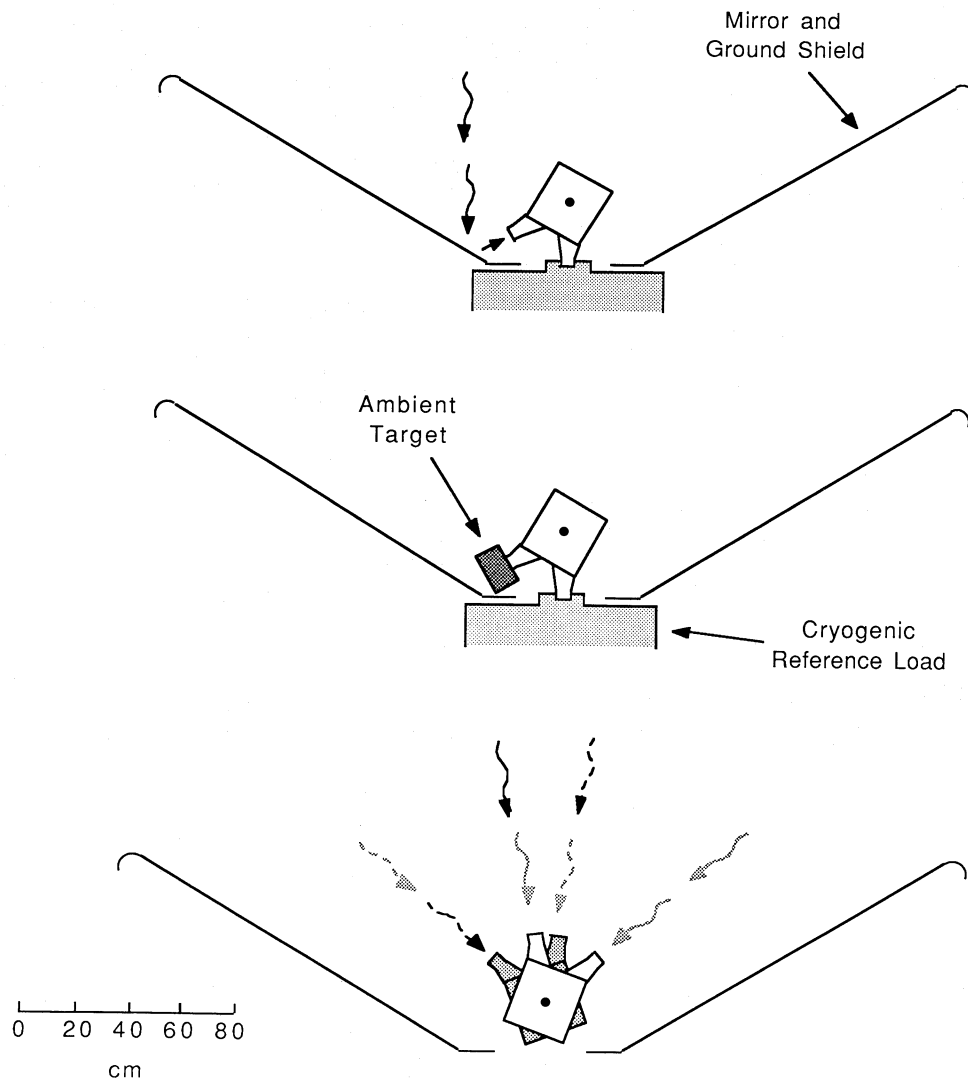
FIG. 1.—The 90 GHz radiometer configuration: (top) zenith sky measurements; (middle) calibration; (bottom) atmospheric scan
